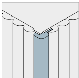
BATTISCOPA - SKIRTING 220 x 45 x 10 mm
